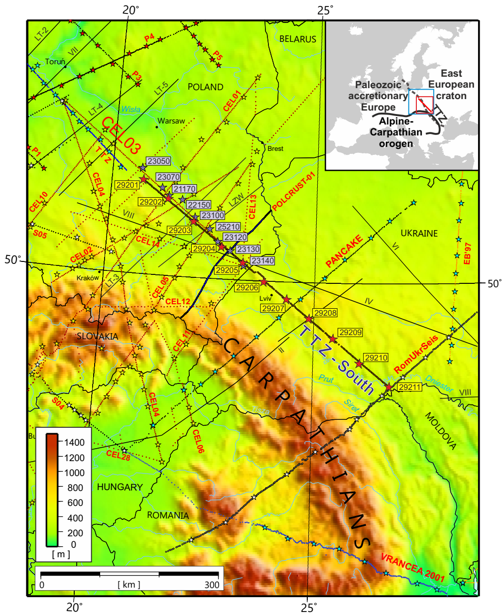
Figure 1. Location of the TTTZ-South, CEL03, TTTZ, PANCAKE, RomUkrSeis, CELEBRATION 2000 (CEL01-CEL16) and other deep seismic sounding (DSS) profiles on a map of Central Europe (red box in the inset map, whereas blue box shows area for whole TTTZ transect). Stars and numbers refer to the locations of shot points along the transect TTTZ-CEL03-TTTZ-South. The beginning of the transect corresponds to the coast of the Baltic Sea (not seen on the map). TTTZ – Teisseyre-Tornquist zone.
